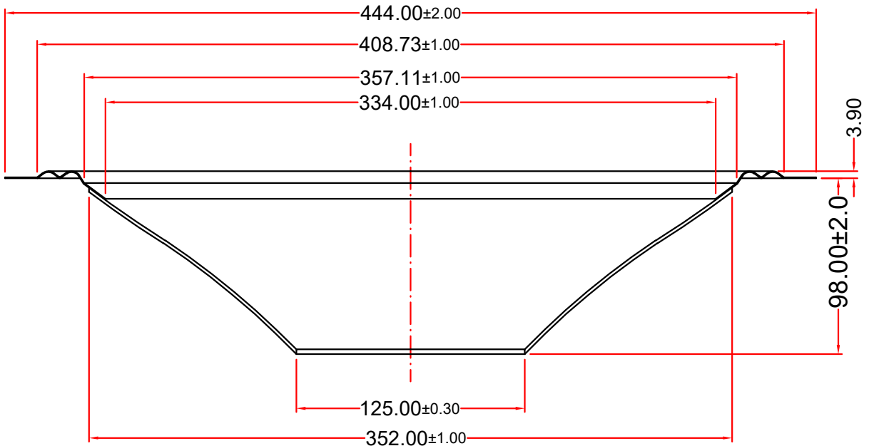
PA-450W-10
